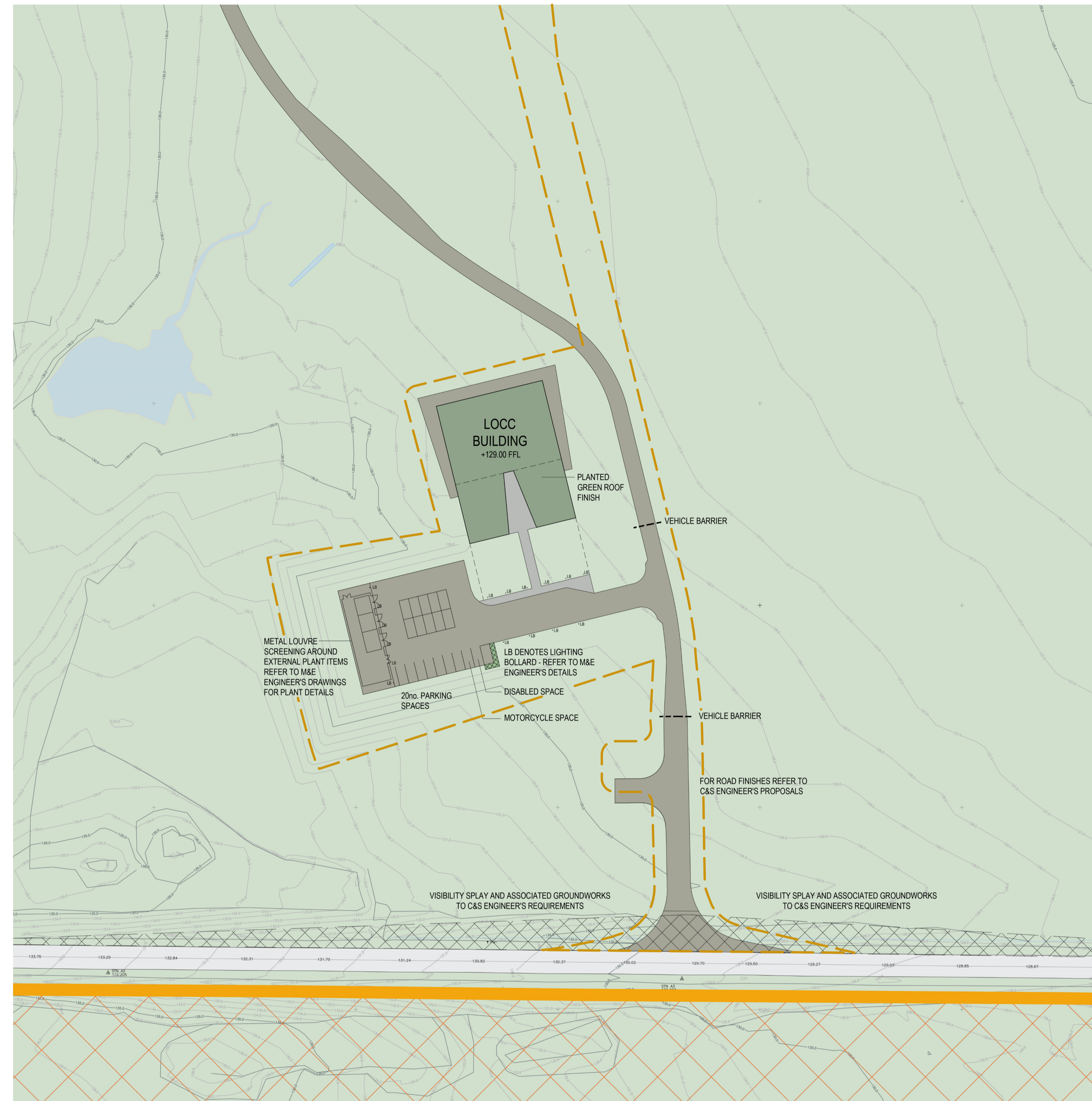
DRAWING EXTRACT - LOCC SITE PLAN AS PROPOSED - NO CHANGE FROM APPROVED SCHEME
